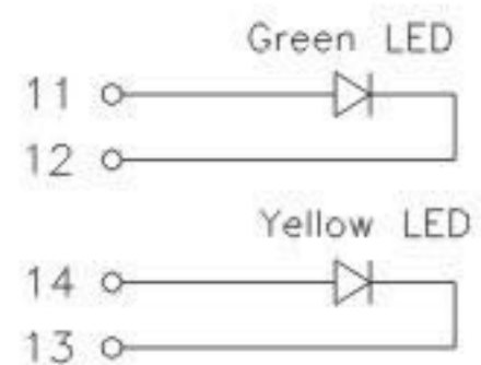
10 PIN
